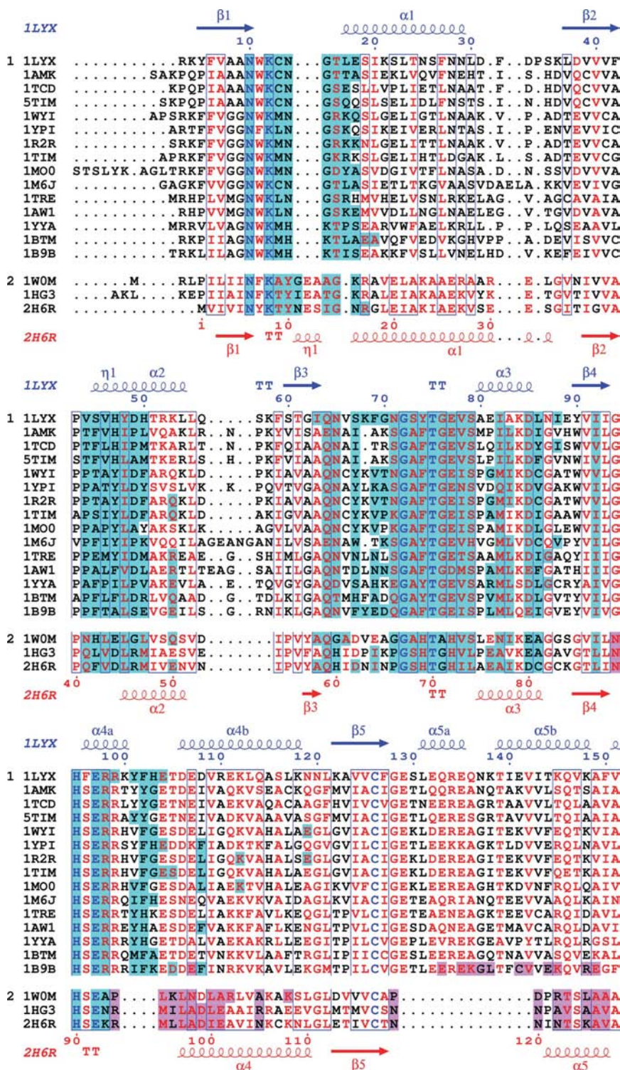
Figure 5 Structure-based sequence alignment of TIMs from various organisms. The structures used to obtain the alignment are denoted by their PDB codes and the details are shown in Table 3. The sequence numbering and secondary-structure assignments at the top (shown in blue) and bottom (in red) correspond to the PwTIM and MjTIM sequences, respectively. The residues involved in dimer and tetramer interfaces are highlighted in cyan and pink, respectively. The three tetrameric TIMs from archaea are grouped together as a separate block from the rest of the TIM sequences. The loop 6 residues in MjTIM, which are missing in the structure, have been included in the alignment according to the pairwise sequence alignment with PwTIM and are highlighted in cyan letters. The structure-based alignment was performed using MUSTANG (Konagurthu et al. , 2006) and represented using ESPrInt (Gouet et al. , 1999). The residues involved in the interfaces were identified using the PISA server (Krissinel & Henrick, 2005) and are highlighted in the representation.
