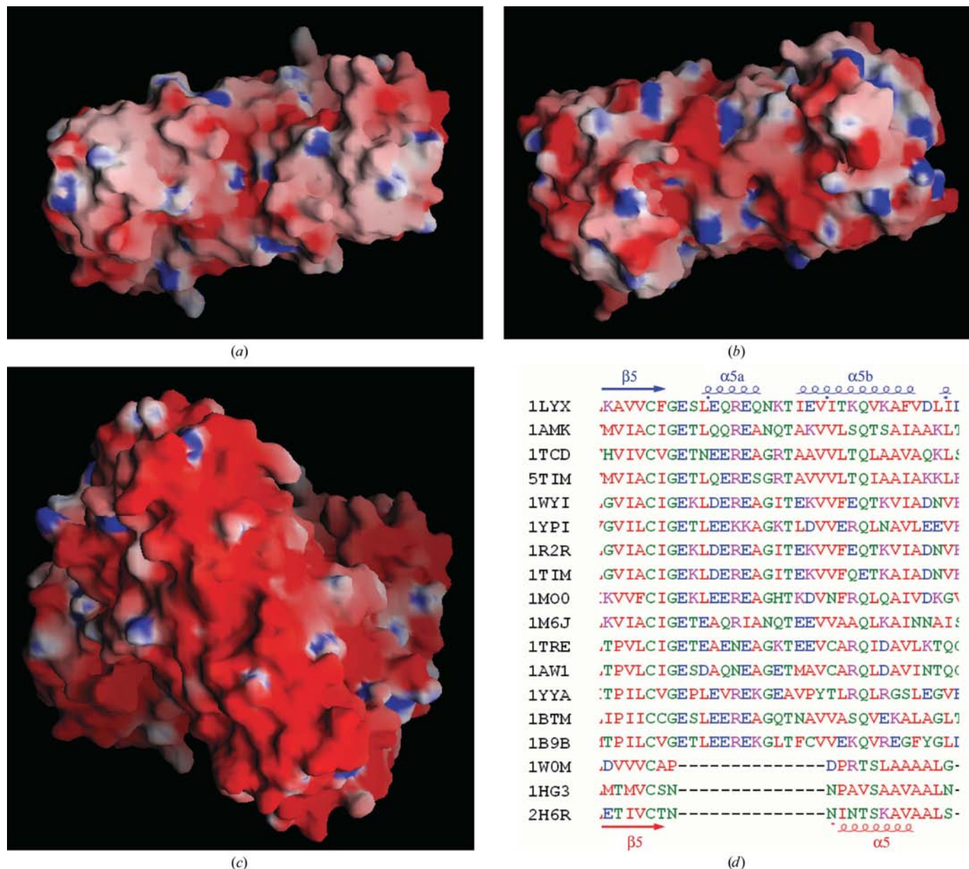
Figure 7 Electrostatic surface-potential representation of dimeric and tetrameric TIMs. (a) MjTIM dimer, (b) PfTIM dimer, (c) MjTIM tetramer. MjTIM and PfTIM dimers are shown in the same orientation, with the tetrameric interface of MjTIM facing towards the viewer. The tetramer is also represented in the same orientation. The figures were generated using GRASP (Nicholls et al. , 1991). Blue, red and white regions represent positively charged, negatively charged and hydrophobic regions respectively. (d) A section of the structure-based sequence alignment of all TIMs, showing the insertion region in the vicinity of helix 5. Acidic residues are coloured blue, hydrophobic red, basic magenta and polar amino acids with hydroxyl and/or amide groups green.
